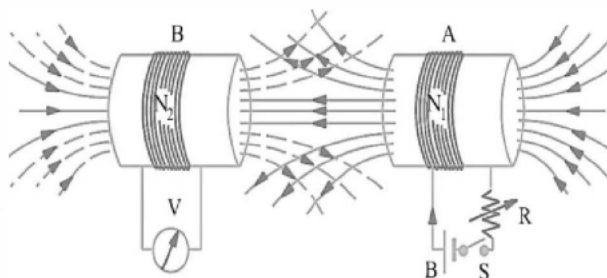
Figure 19.8 Mutual Inductance
