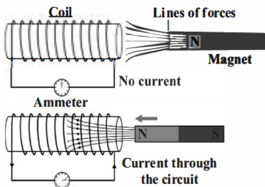
Figure 19.3 Electromagnetic induction
