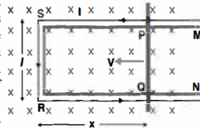
Figure 19.11 Motional emf
